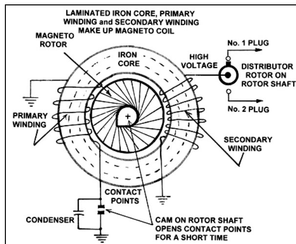
Figure 705. Magneto Ignition System
